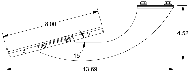
SIDE VIEW
