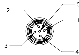
DETAIL A SCALE 1 : 1 PINOUT DETAIL
