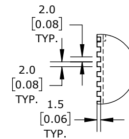
DETAIL A SCALE 2 : 3
