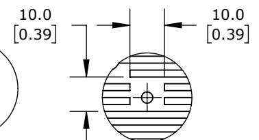
DETAIL B SCALE 2 : 3
