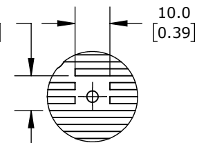
DETAIL B SCALE 2 : 3
