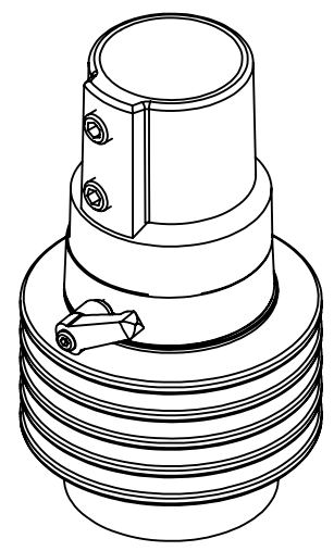
ISOMETRIC VIEW
