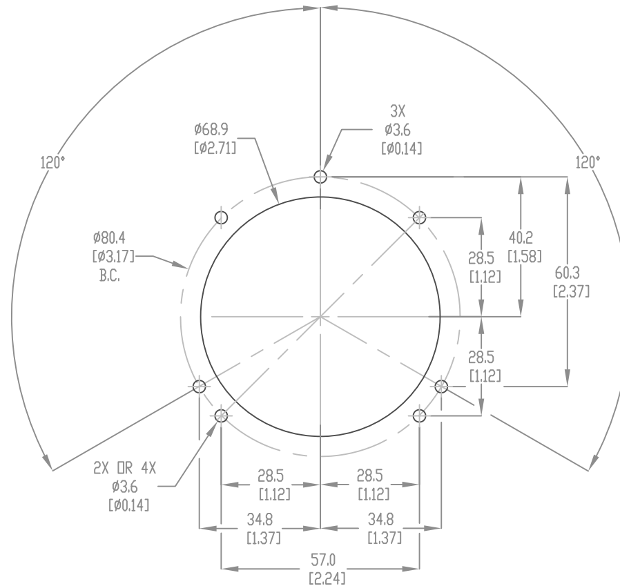
3 STUD FIXING MOUNT 120° EQUALLY SPACED ON Ø80.4mm B.C.
