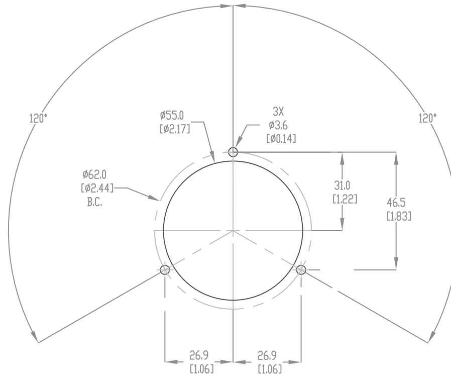
3 STUD FIXING MOUNT 120° EQUALLY SPACED ON Ø62.0mm B.C.
