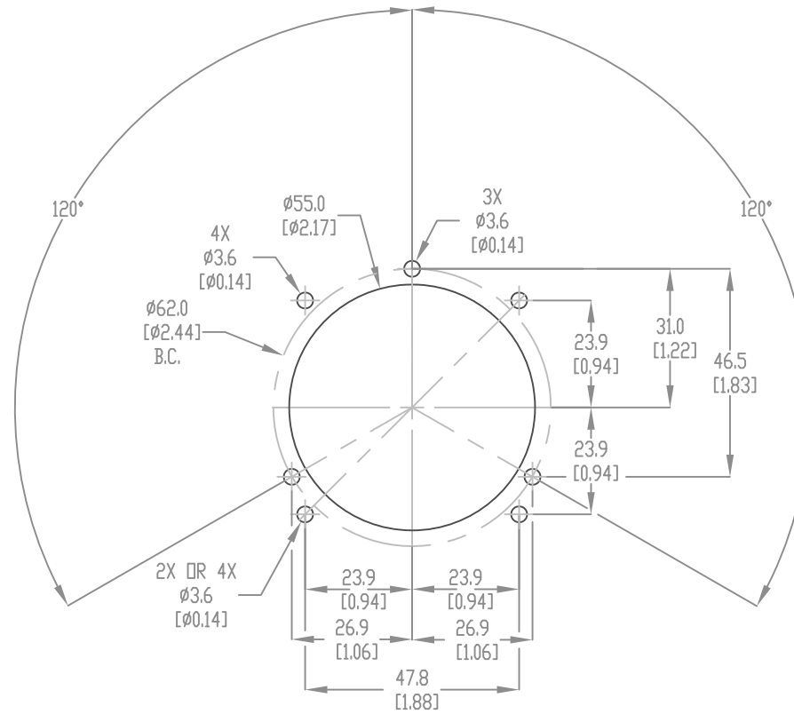
3 STUD FIXING MOUNT 120° EQUALLY SPACED ON Ø62.0mm B.C.
