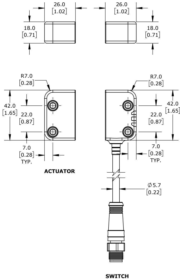
SWITCH CONNECTOR
