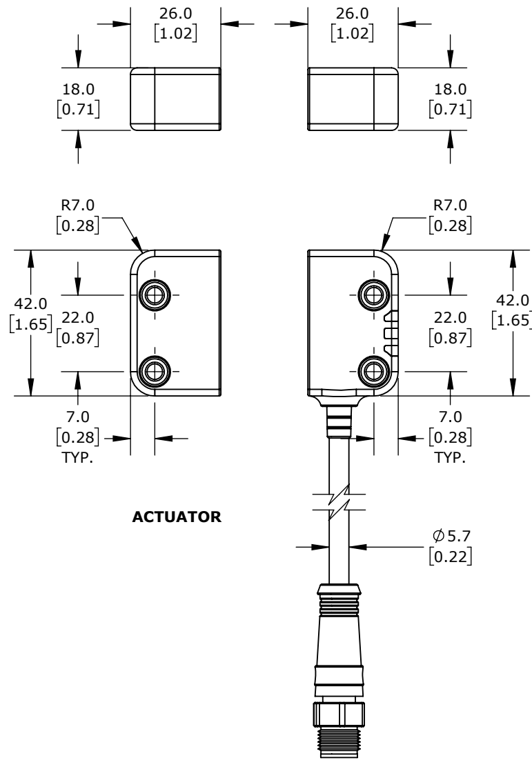
SWITCH
