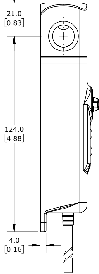
SWITCH
