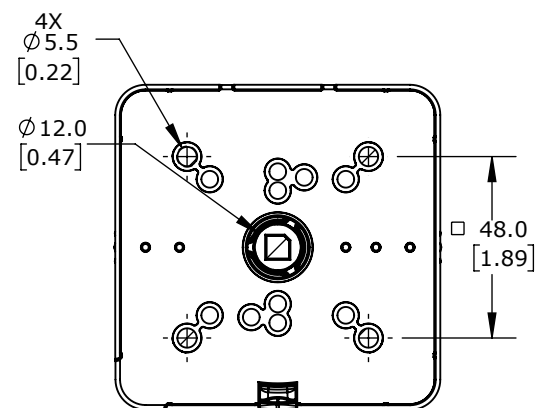
SECTION A-A MOUNT TEMPLATE DIMENSIONS
