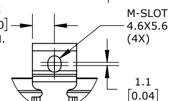
DETAIL A SCALE 2 : 2.5
