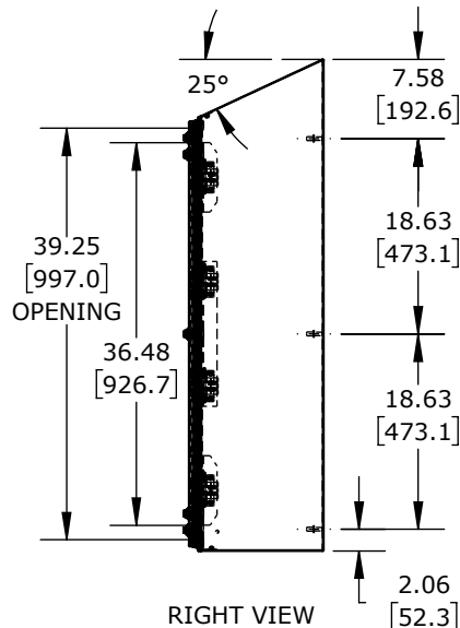
RIGHT VIEW
