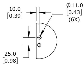
DETAIL A SCALE 1 : 6
