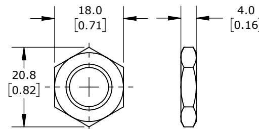
M12X1.0 HEX NUT DETAIL VIEW
