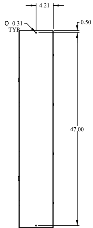
BOTTOM VIEW
