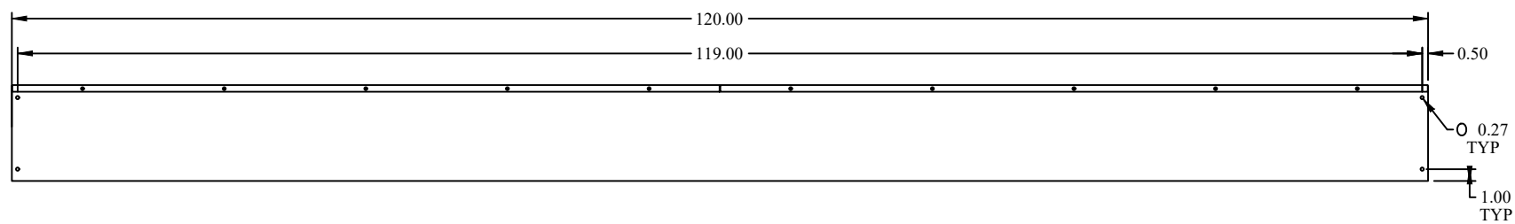
SIDE VIEW
