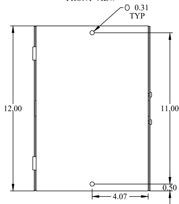
BOTTOM VIEW
