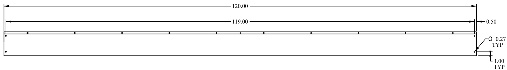
SIDE VIEW
