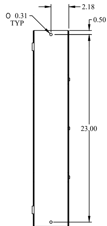
BOTTOM VIEW
