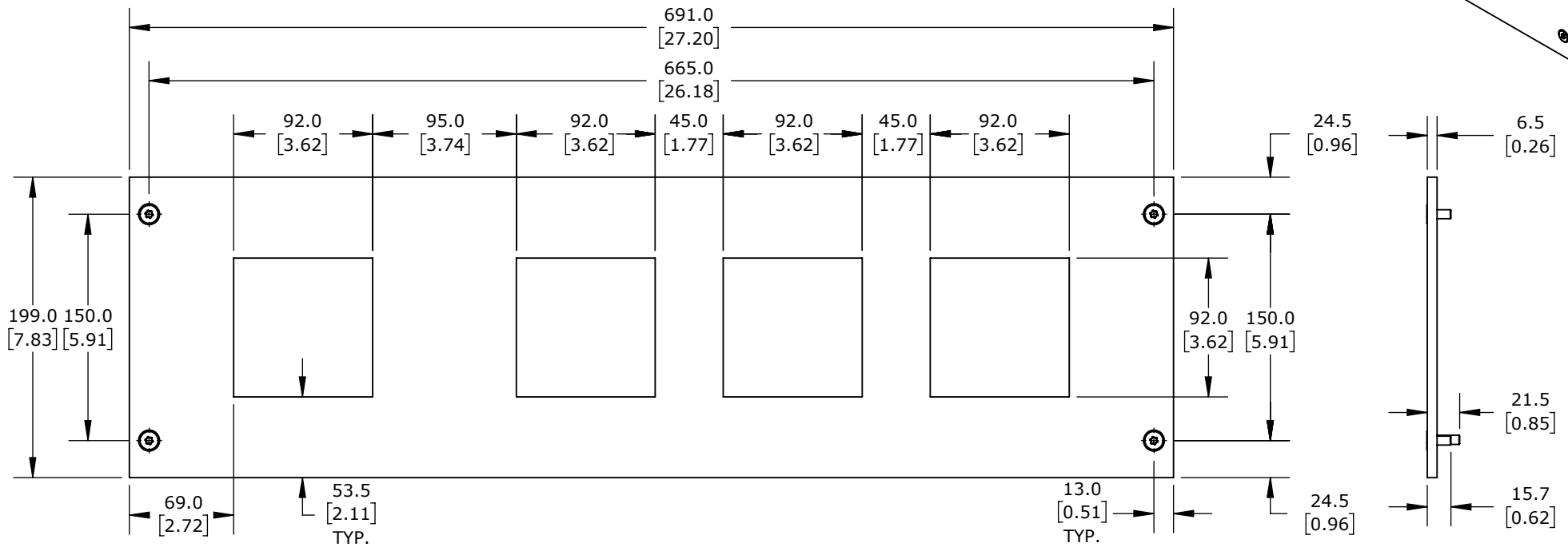
ISOMETRIC VIEW
