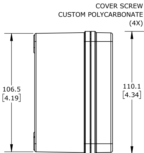
DETAIL C
