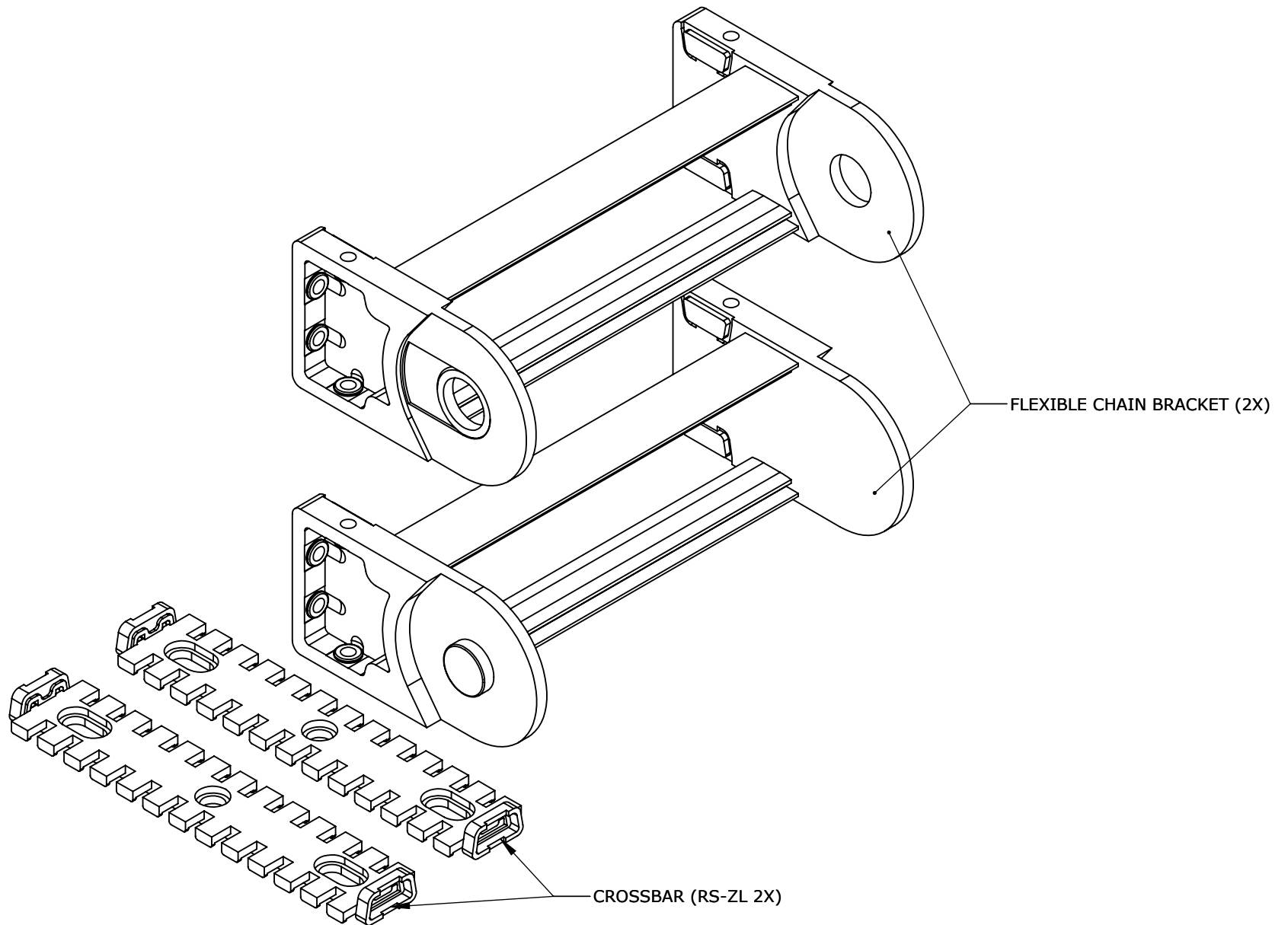
ISOMETRIC VIEW
