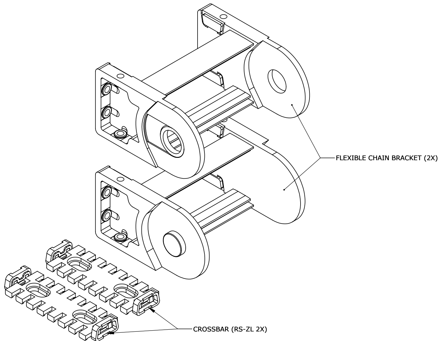
ISOMETRIC VIEW
