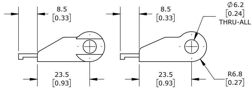
MALE BRACKET
