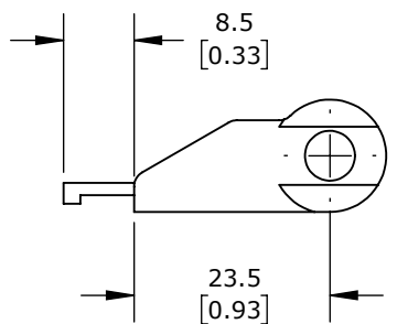
MALE BRACKET
