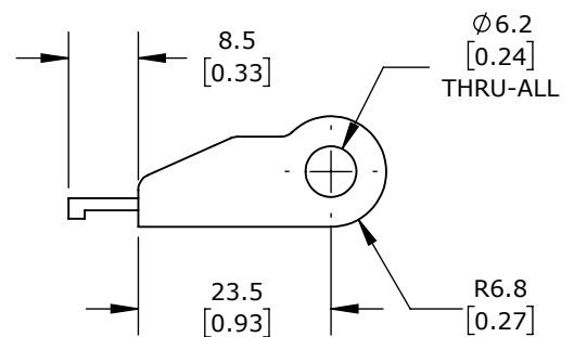
FEMALE BRACKET
