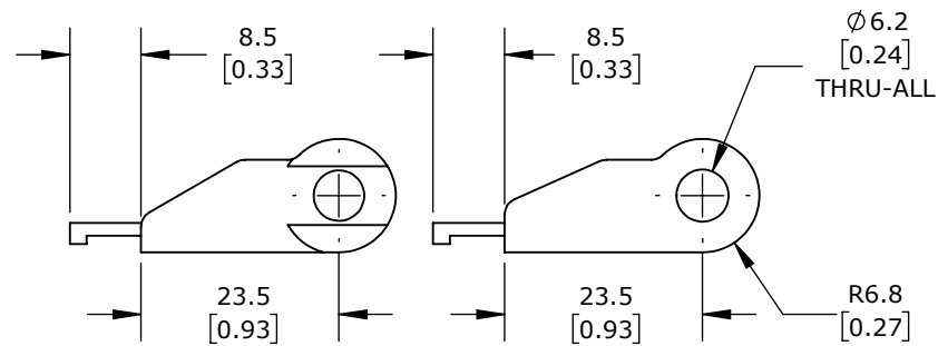
MALE BRACKET
