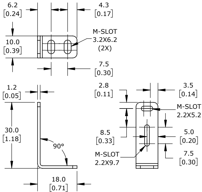
MOUNTING BRACKET ( 2 PIECE )
