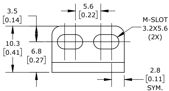
MOUNTING BRACKET
