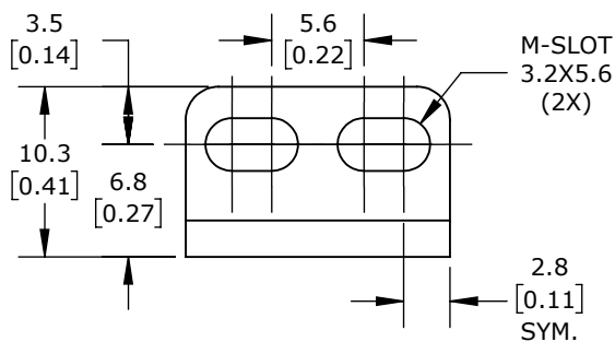
MOUNTING BRACKET
