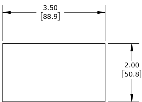
SAE O-RING BOSS (ORB) #8 PORTS X4
