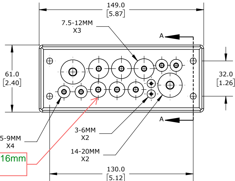
PANEL CUTOUT DETAIL
