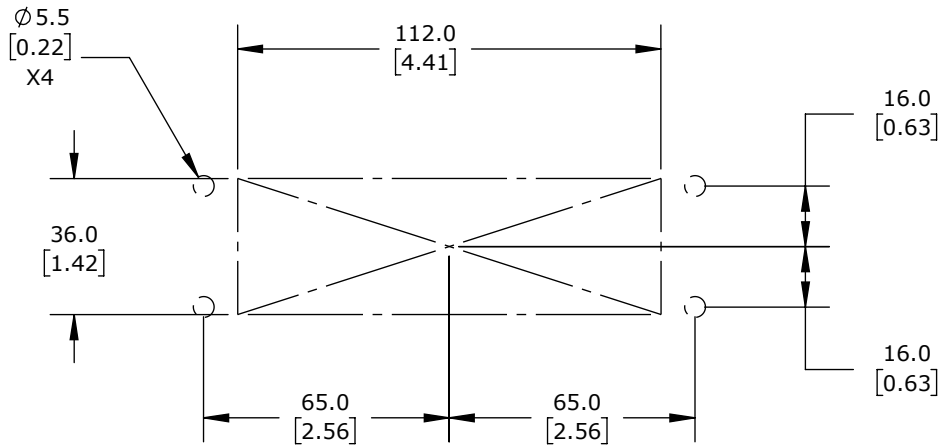
PANEL CUTOUT DETAIL
