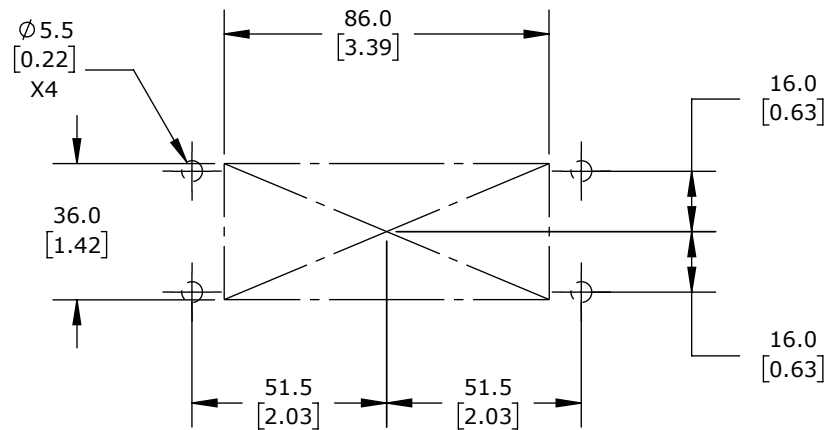
PANEL CUTOUT DETAIL
