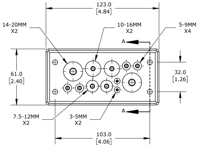
PANEL CUTOUT DETAIL
