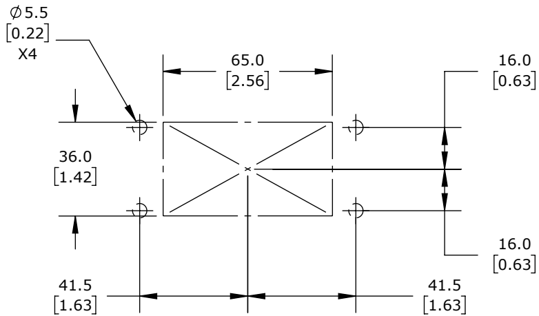
PANEL CUTOUT DETAIL
