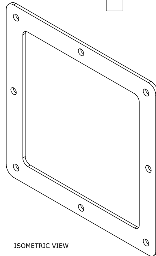
WIREWAY GASKET KIT (FOR USE WITH 1487 SERIES WIREWAY)
