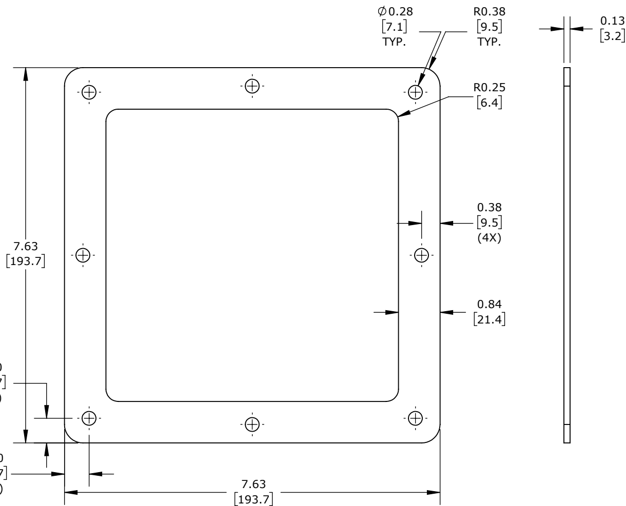
WIREWAY GASKET KIT (FOR USE WITH 1487 SERIES WIREWAY)
