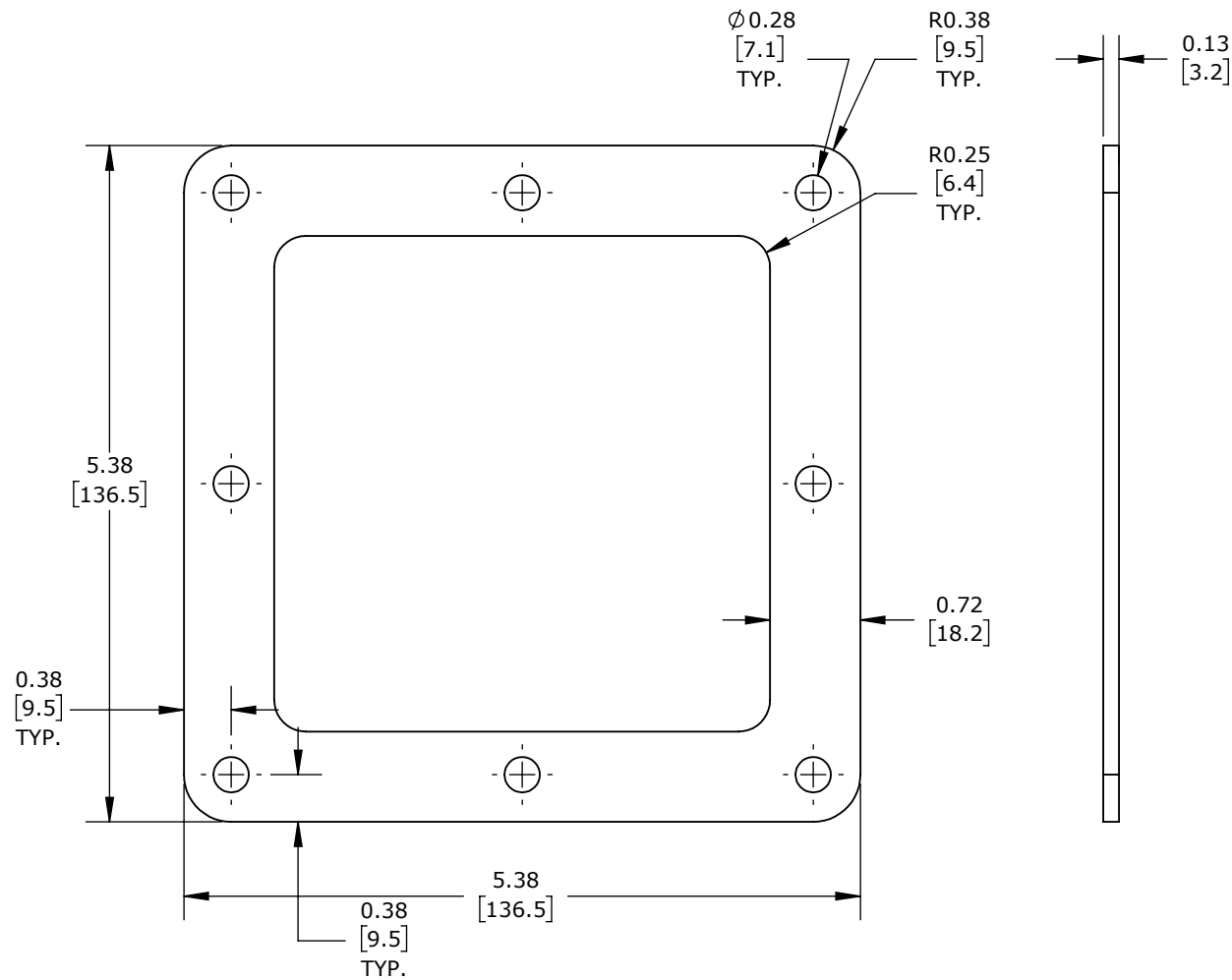
FRONT VIEW
