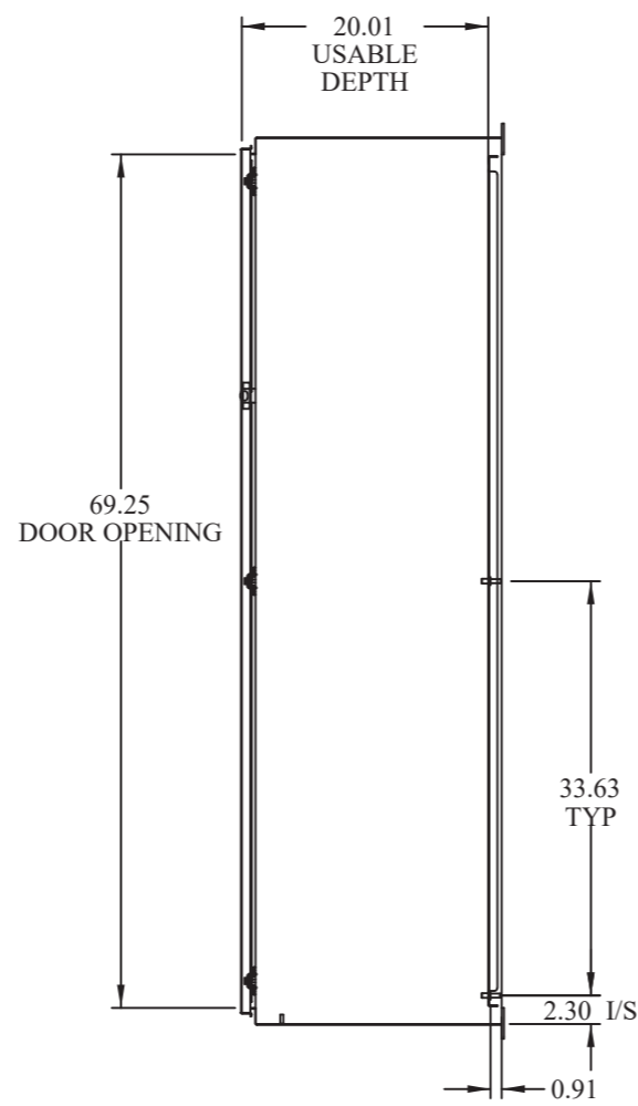
SIDE VIEW
