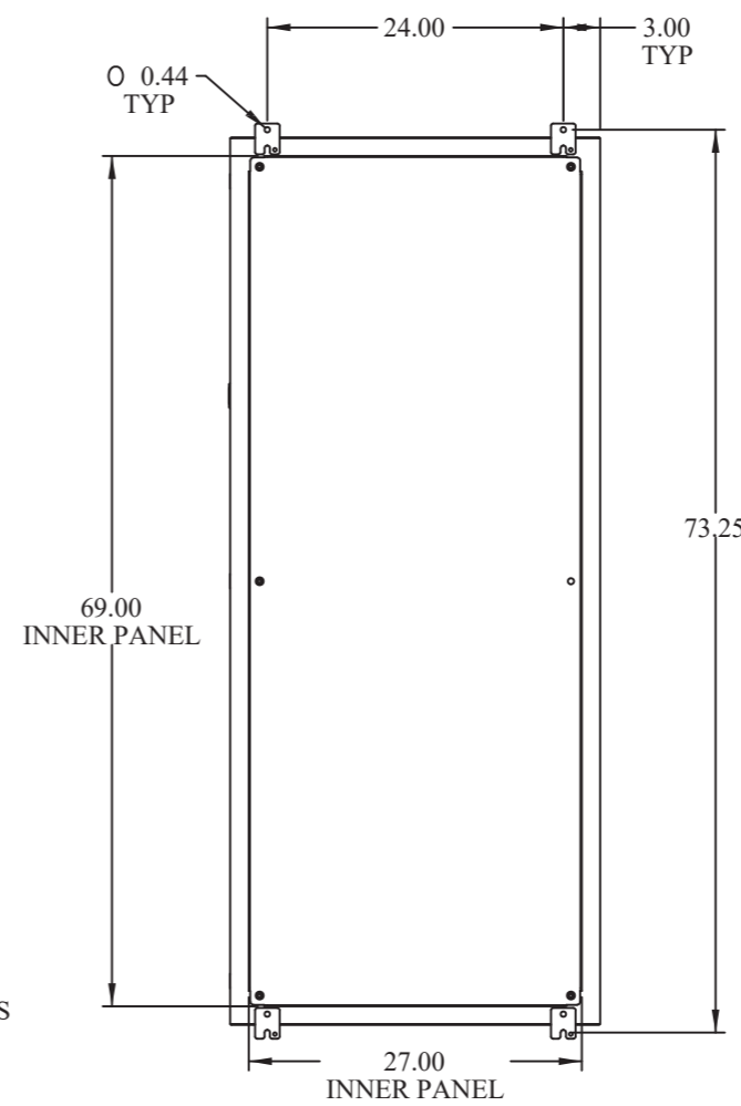
BACK VIEW
