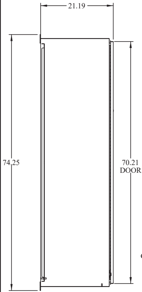
SIDE VIEW
