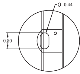
DETAIL Z
