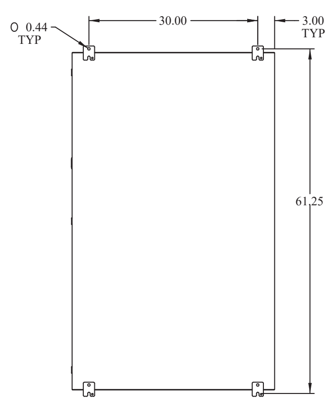
BACK VIEW
