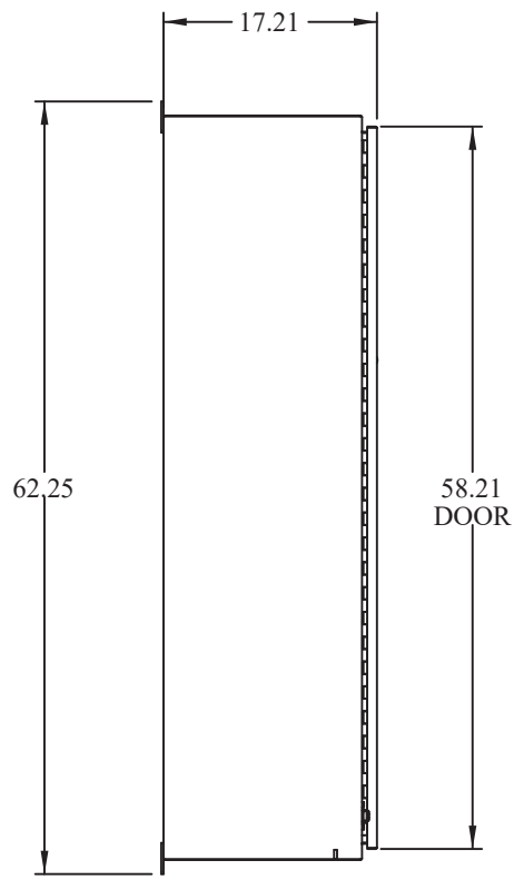
SIDE VIEW
