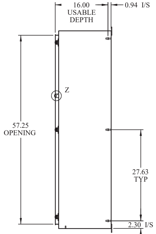
SIDE VIEW (DOOR REMOVED)
