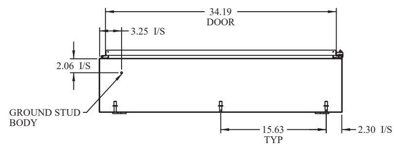
BOTTOM VIEW
