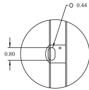
DETAIL Z
