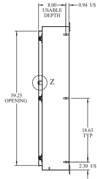
SIDE VIEW (DOOR REMOVED)
