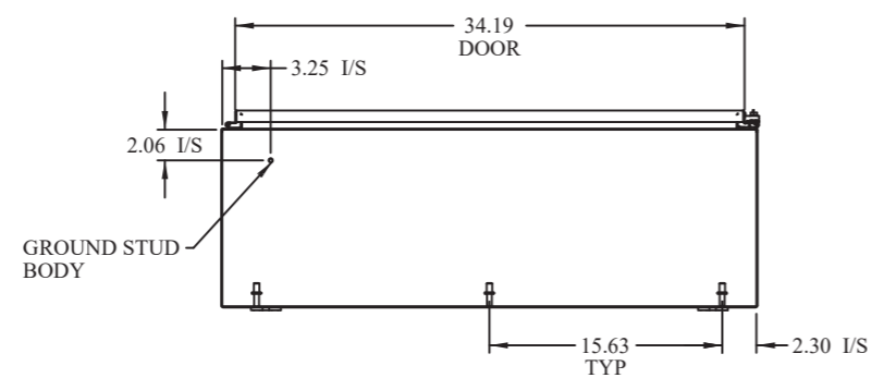
BOTTOM VIEW
