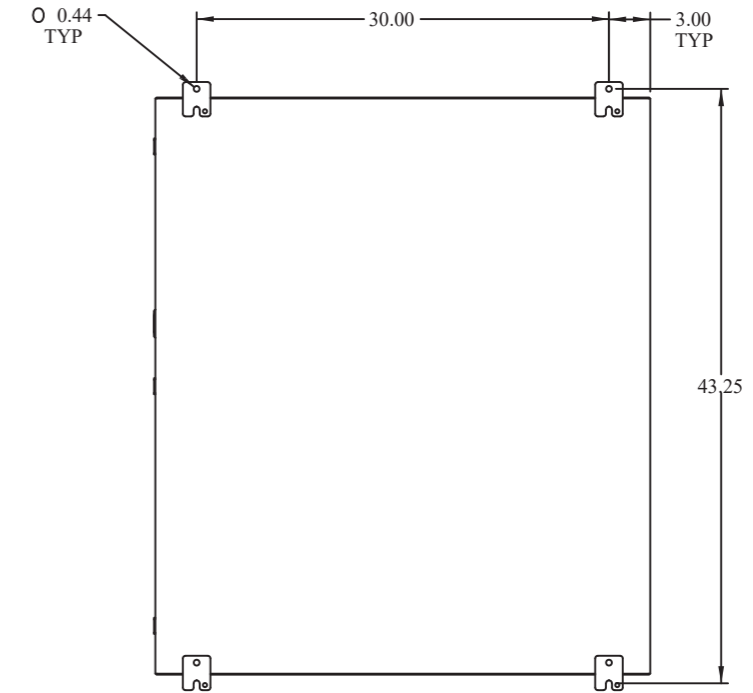
BACK VIEW
