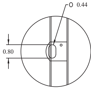
DETAIL Z
