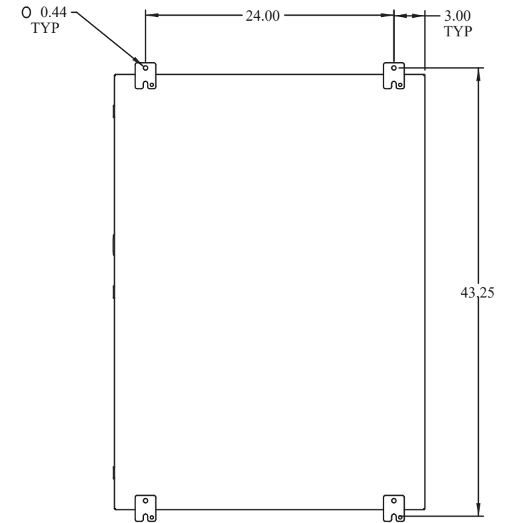
BACK VIEW
