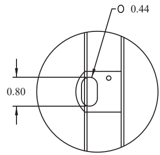
DETAIL Z
