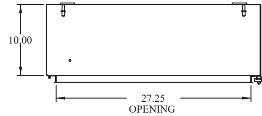
TOP VIEW (DOOR REMOVED)
