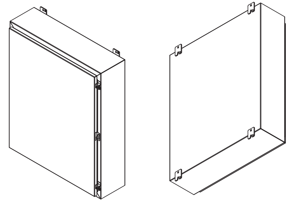
ISOMETRIC VIEWS
