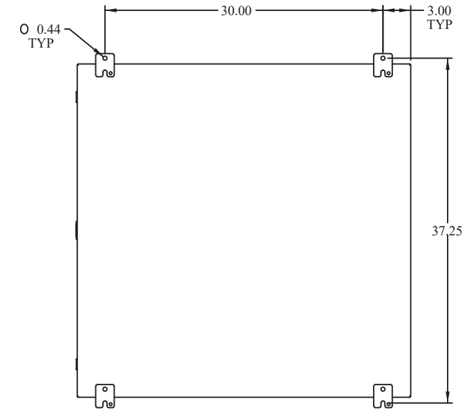
BACK VIEW
