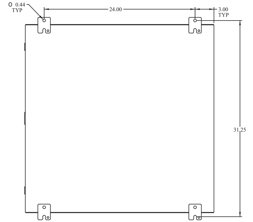
BACK VIEW
