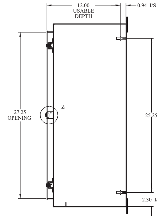
SIDE VIEW (DOOR REMOVED)
