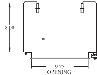
TOP VIEW (DOOR REMOVED)
