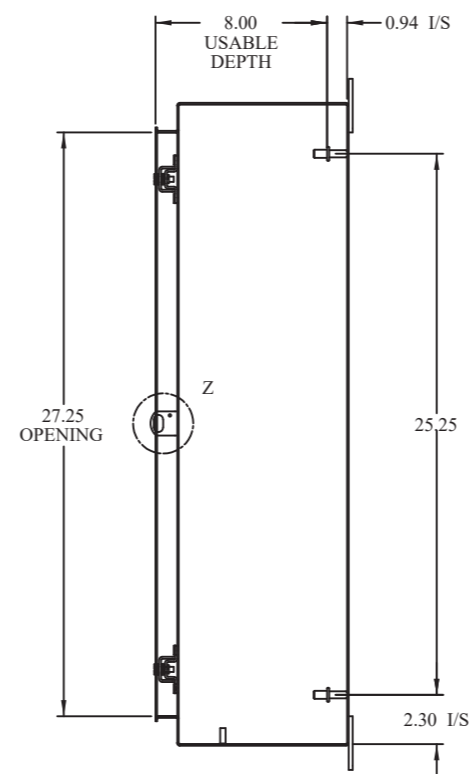
SIDE VIEW (DOOR REMOVED)
