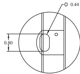
DETAIL Z
